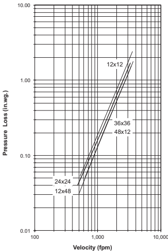
Figure 5.2 — Ducted Inlet
