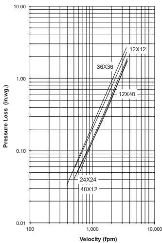
Figure 5.5 Plenum Mount
