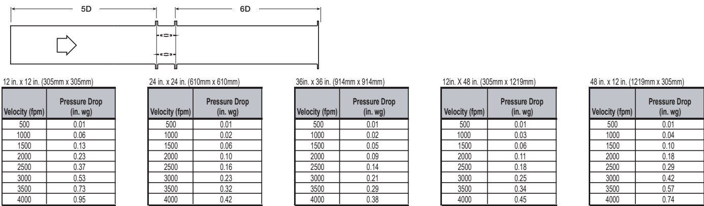
AMCA Figure 5.5
