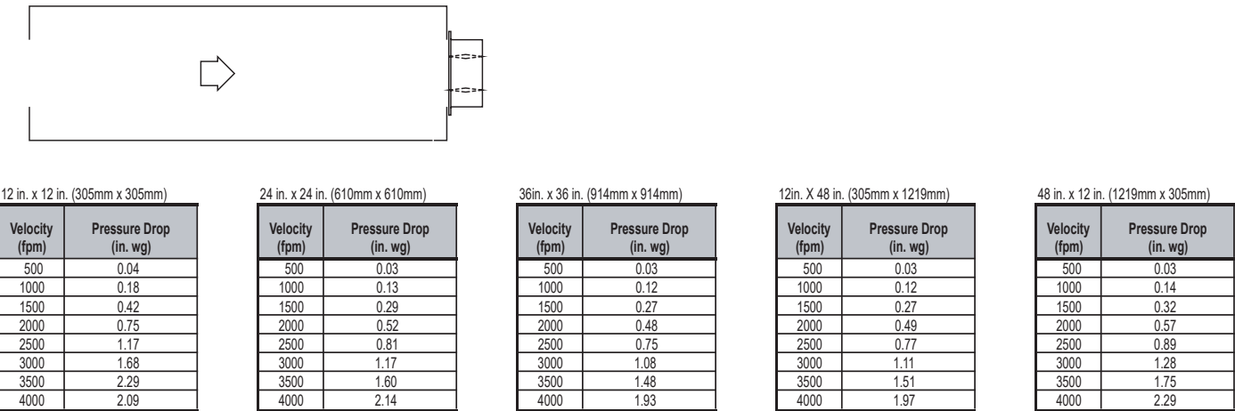
AMCA Figure 5.5
