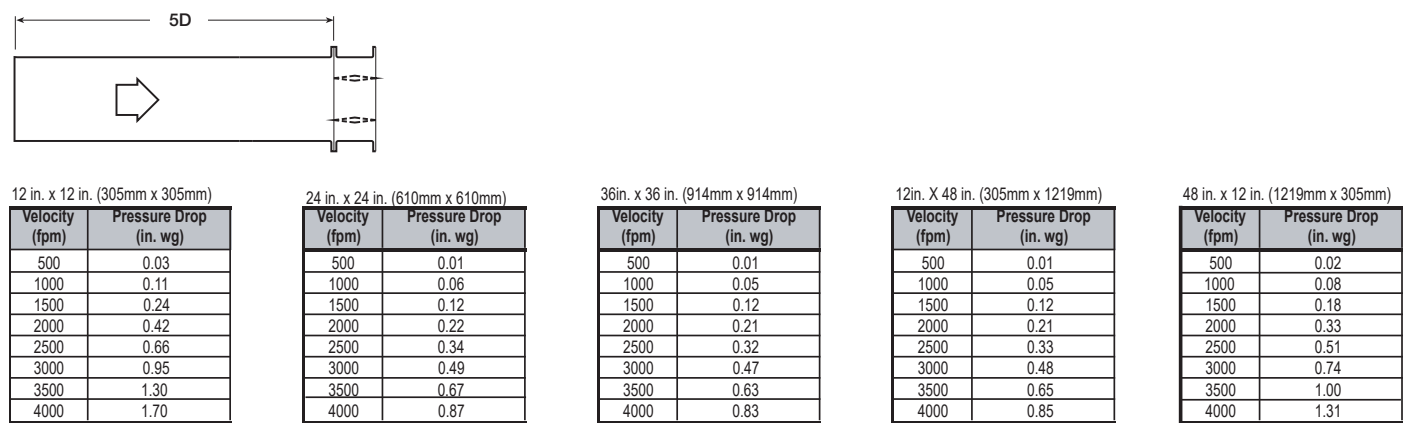
AMCA Figure 5.3
