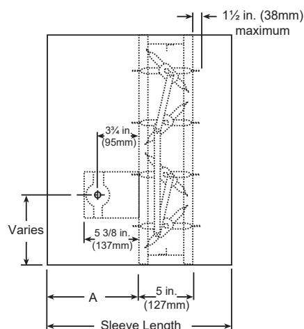
Sleeve
