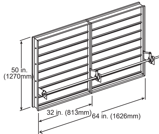
Two Section
