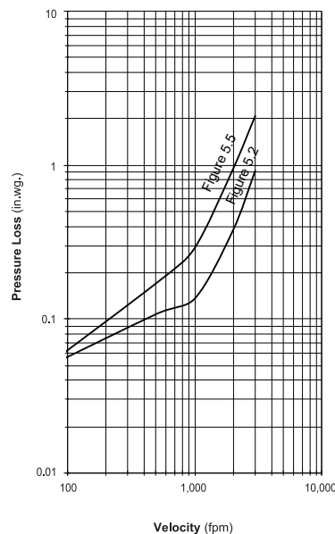
Pressure Drop vs. Velocity 24" x 24" Damper
