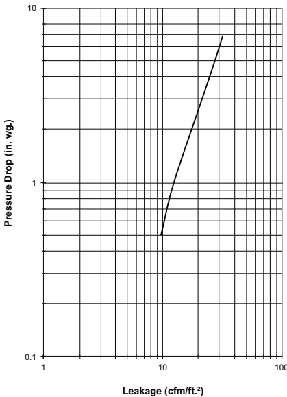
Leakage vs. Pressure Drop 24" x 24" Damper
