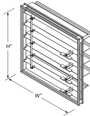
Model CBD-250 (standard) * Damper dimensions furnished approximately 1/4" (6) undersize.
