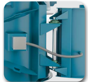
Swingout Construction
