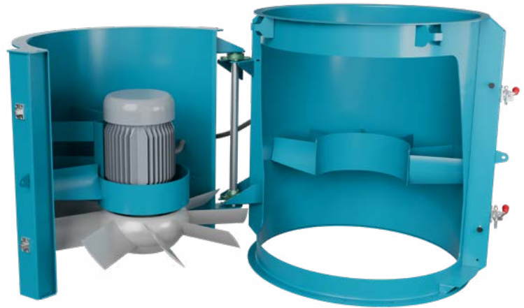
Swingout Construction
