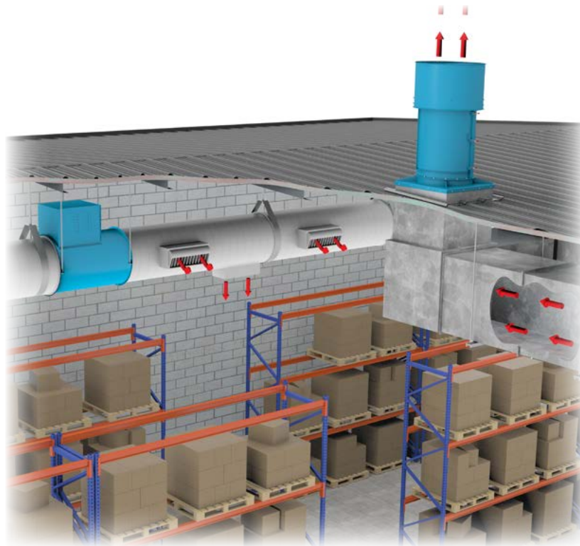
Warehouse Application with VRM & HCH Fans
