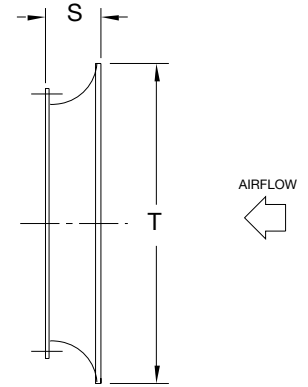
INLET BELL
