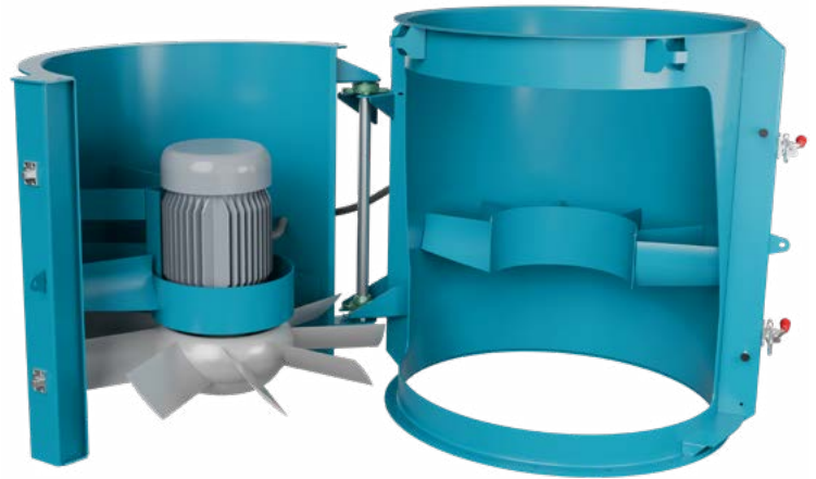
Swingout Construction
