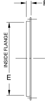
COMPANION FLANGE
