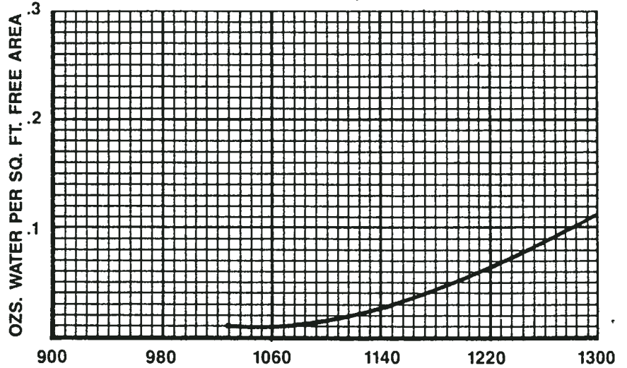
FREE AREA VELOCITY F.P.M.
