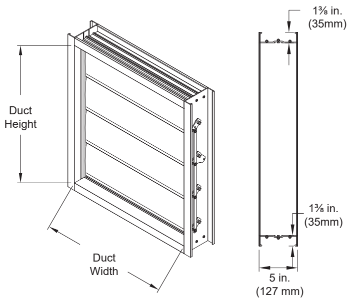
Quick Connect
