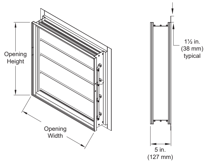
Reverse Flange
