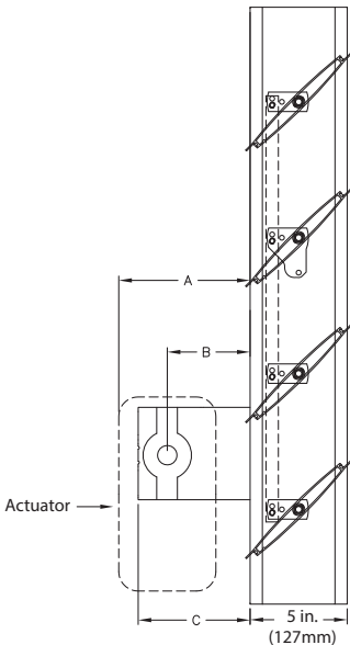
This drawing depicts the worst case clearance requirements for an actuator with a jackshaft.
