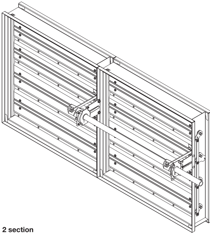
2 section
