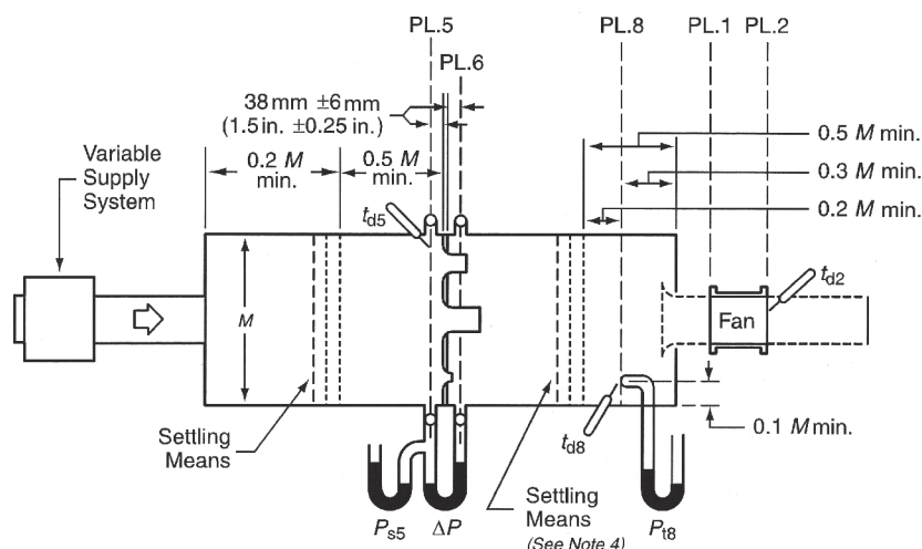
Figure 15 - Inlet chamber Setup - Multiple Nozzles In Chamber (ANSI / AMCA 210- ANSI / ASHRAE 51)
