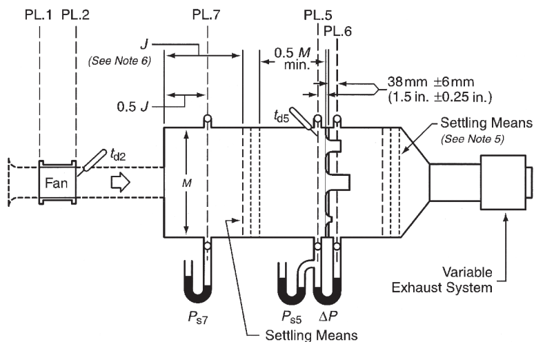
Figure 15 - Inlet chamber Setup - Multiple Nozzles In Chamber (ANSI / AMCA 210- ANSI / ASHRAE 51)
