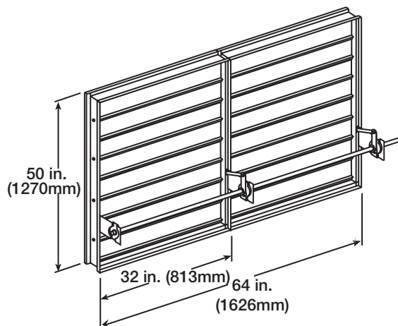
Two Section
