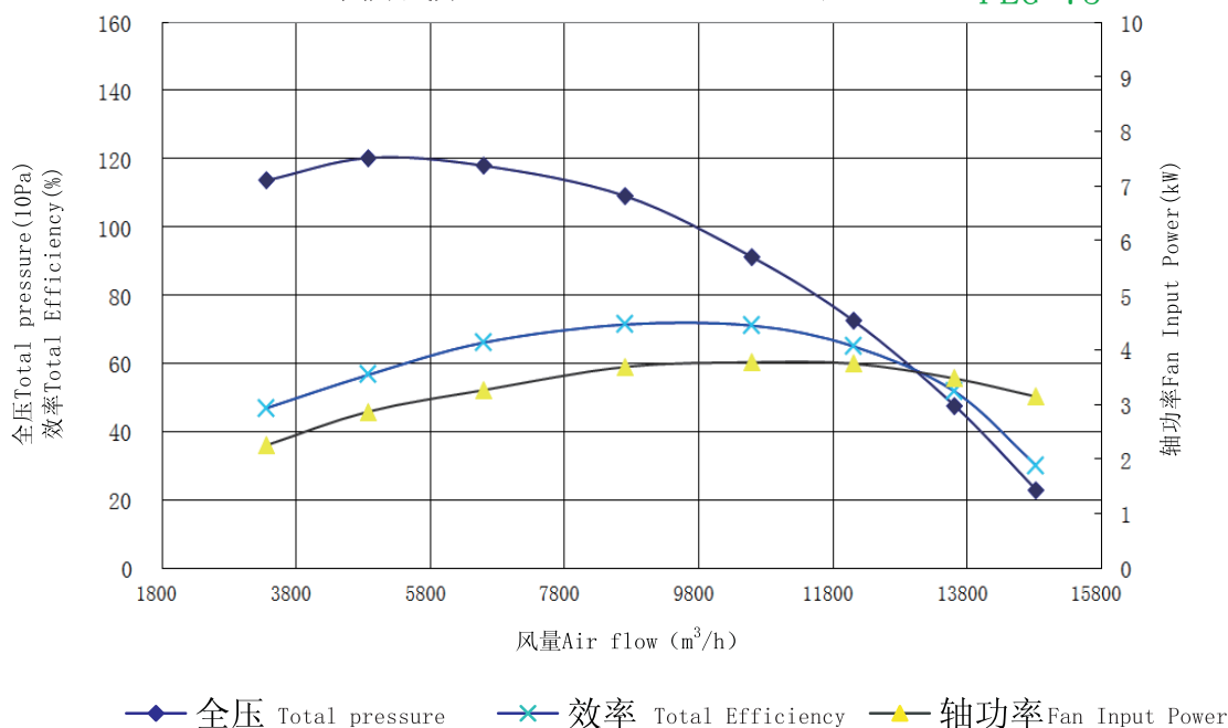
4-79-6A性能曲线图 (Performance curve) n=1450r/min
