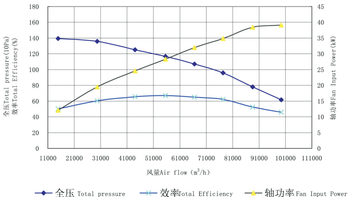
4-79-14E性能曲线图 (Performance curve) n=680\text{r/min}
