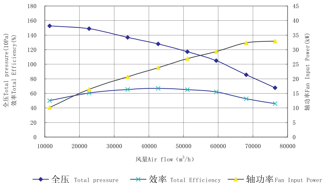
4-79-12E性能曲线图 (Performance curve) n=830\text{r/min}
