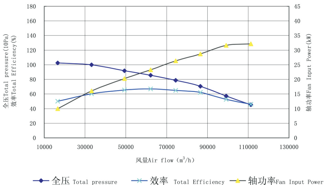
4-79-16E性能曲线图 (Performance curve) n=510\text{r/min}
