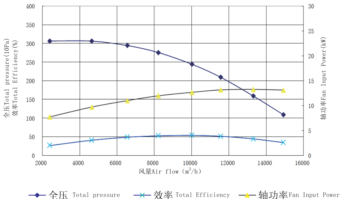
4-79-5A性能曲线图 (Performance curve) n=2900r/min
