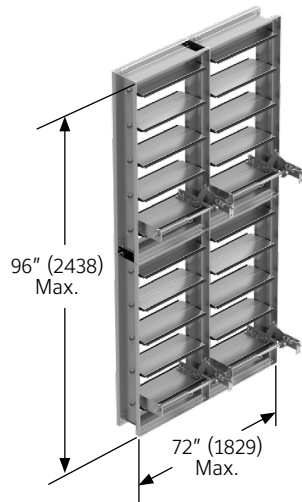
DFD60 MULTIPLE SECTION
