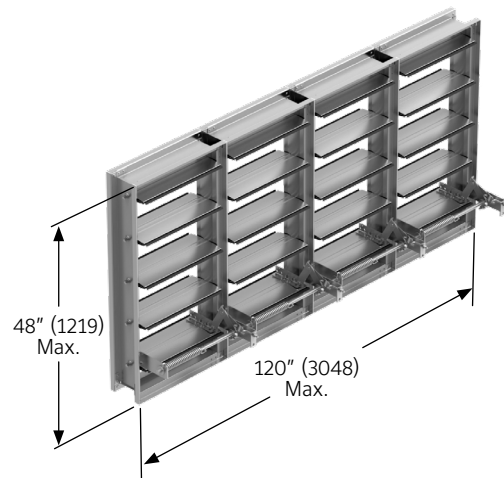
DFD60 MULTIPLE SECTION
