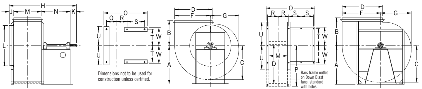
DIMENSIONS [INCHES]
